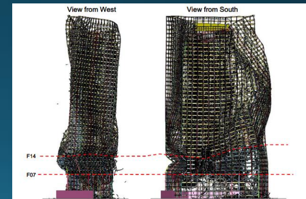
Figure 4-47. Global model with lateral displacement contours (-1 m to 1 m) at 8.6 (24.6) s.
